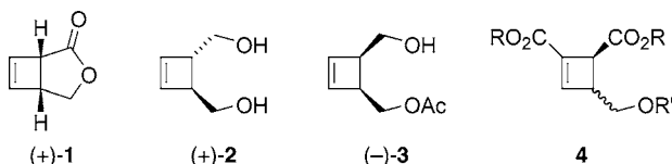
Figure 1. Synthetically useful cyclobutene derivatives.
