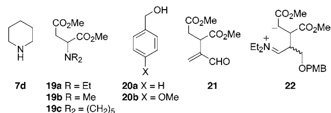
Figure 2. Structures relating to Table 1 and other experiments.
