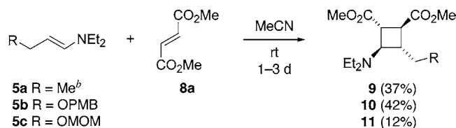
Scheme 1. Reactions of Enamines 5 with Dimethyl Fumarate a
