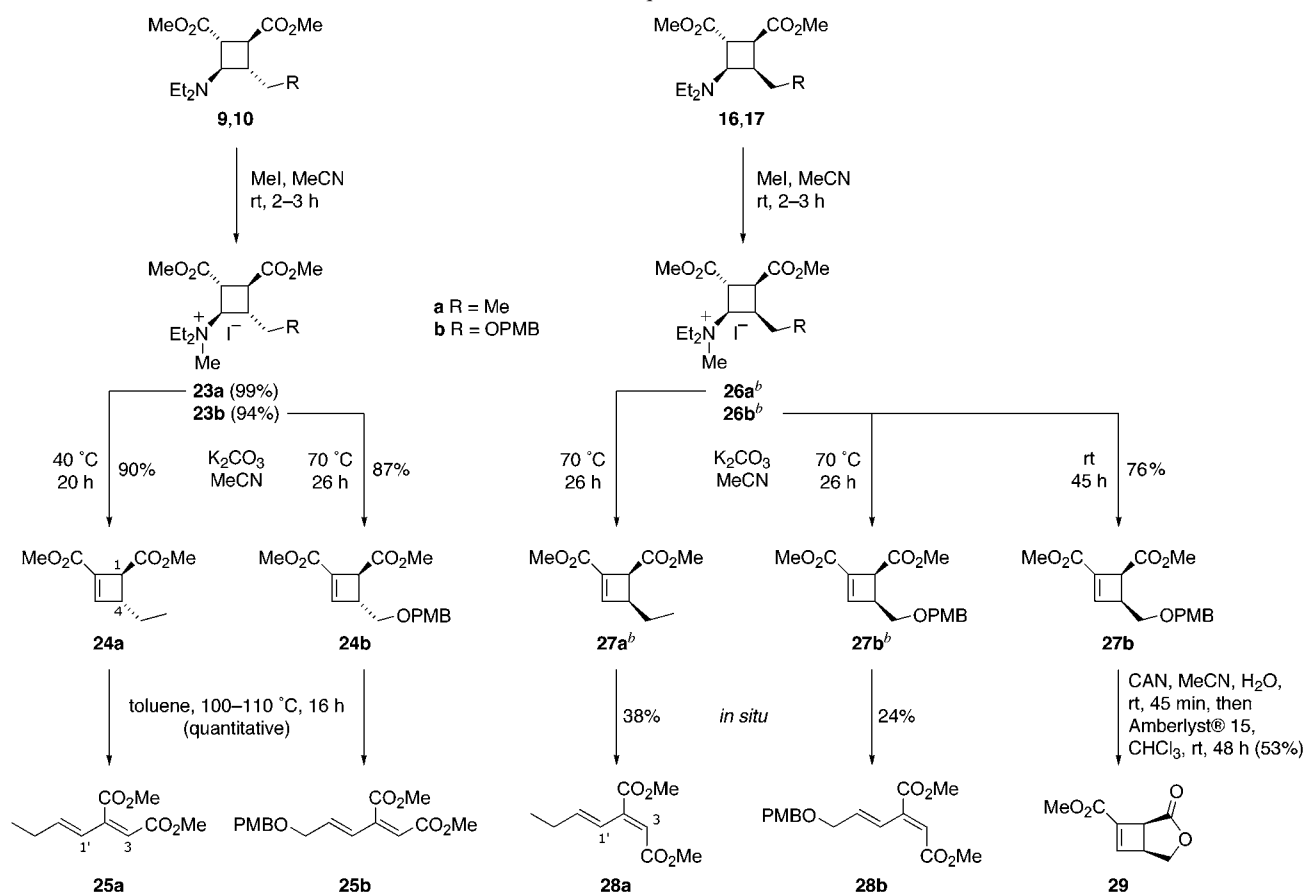
Scheme 2. Elimination Sequences with 9 , 10 , 16 , and 17 a
