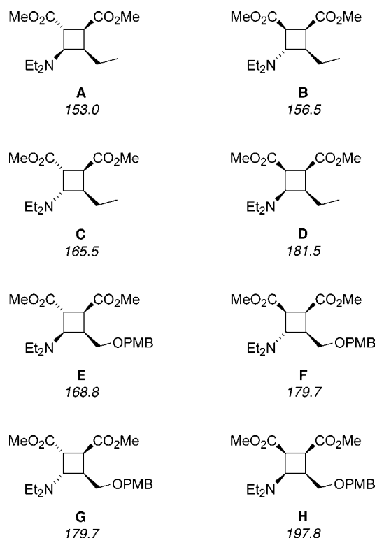
Figure 3. Calculated minimum steric energies (kJ mol -1 ) of the 1,4- cis diastereoisomers of 16 and 17 (Macromodel 8.0, MM3).
